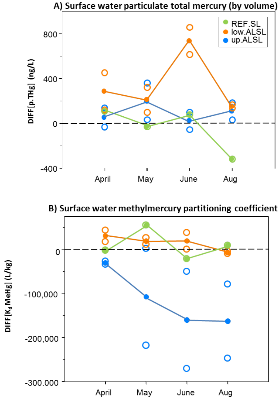
Figure 46. Line graph of the annual difference (DIFF[Y2011 – Y2010]) for mercury parameters in surface water of Sloughs, by MONTH and LOCATION. Open circles represent the original data, while closed circles with lines represent the DIFF-Y model predicted values, where DIFF-Y = MONTH + LOCATION + MONTH*LOCATION . Only cases where a Tukey's family-wise comparison of LOCATION resulted in significant differences ( P < 0.05 ) between the reference location (REF.Slough) and the treatment location (up.ALSL and/or low.ALSL) are depicted. The specific sites associated with each LOCATION grouping are identified in Table 12.
