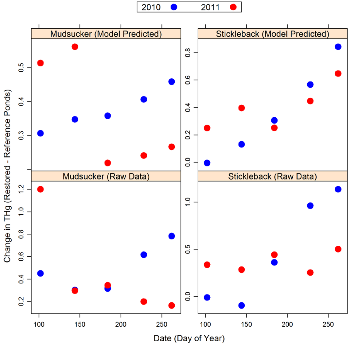
Figure 28. Difference between Restored Pond (A5, A7, and A8) and Reference Pond (A16 and A3N) total mercury (THg) concentrations ( \mu\text{g/g} dry weight) versus sampling time period for pre-restoration (blue: 2010) and post-restoration (red: 2011) in San Francisco Bay, CA. Longjaw Mudsucker data are presented on the left panels and Threespine Stickleback data are presented on the right panels. Raw data are presented on the bottom panels and model predicted data, which account for other variables which influenced total mercury concentrations in fish, are presented on the top panels. Whereas most of the management activities associated with the restoration of the Pond A8/A7/A5 Complex occurred between years of sampling, the Pond A8 Notch was physically opened to tidal influence on June 1, 2011 (day of year = 152), between sampling time periods two and three in 2011. The data show that for both Mudsuckers and Stickleback, fish THg concentrations increased, relative to Reference Ponds, after the restoration activities between years for the first two sampling time periods before the Pond A8 Notch was opened in 2011. However after the Pond A8 Notch was opened, fish THg concentrations declined in Restored Ponds relative to Reference Ponds.
