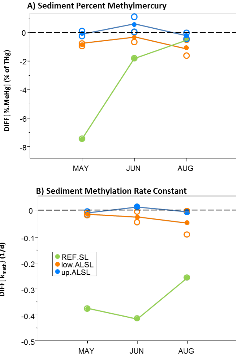
Figure 40. Line graphs of the annual difference (DIFF[Y2011 – Y2010]) for mercury parameters in surface sediment of Sloughs, by MONTH and LOCATION. Open circles represent the original data, while closed circles with lines represent the DIFF-Y model predicted values, where DIFF-Y = MONTH + LOCATION + MONTH*LOCATION . Only cases where a Tukey's family-wise comparison of LOCATION resulted in significant differences ( P < 0.05 ) between the reference location (REF.Slough) and the treatment location (up.ALSL and/or low.ALSL) are depicted. The specific sites associated with each LOCATION grouping are identified in Table 10. The results indicate that for at least one of the sampling months the interannual variability in both sediment %MeHg and k_{meth} was significantly different between the REF.SL and the two Alviso Slough LOCATIONS. Specifically, both sediment parameters measurably decreased in the REF.SL between 2010 and 2011, but not in either of the two Alviso Slough LOCATIONS.
