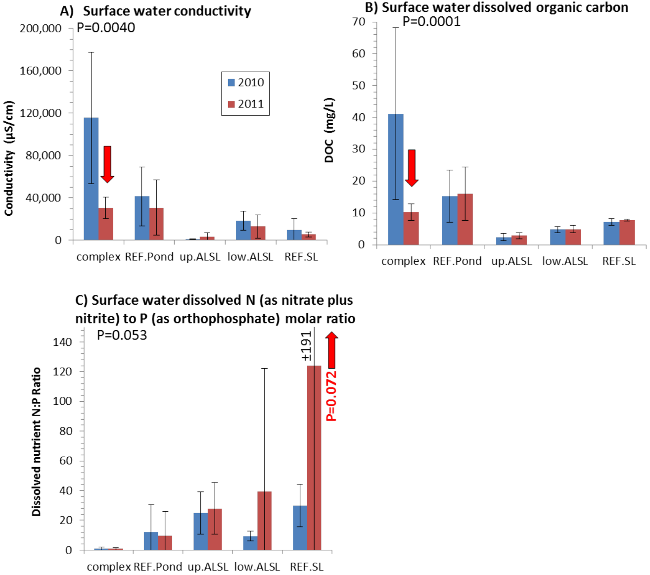
Figure 44. Bar graphs of aqueous non-mercury parameters in surface water by YEAR and LOCATION. Colored bars represent the mean and error bars represent the standard deviation. The statistical Probability (P) value associated with the global model YEAR*LOCATION interaction term is given for each parameter plot. Statistically significant differences ( P < 0.05 , unless otherwise noted) between YEARS for an individual LOCATION is indicated by the red arrow, as either an increase (up arrow) or decrease (down arrow) from 2010 to 2011. The specific sites associated with each LOCATION grouping are identified in Table 12.
