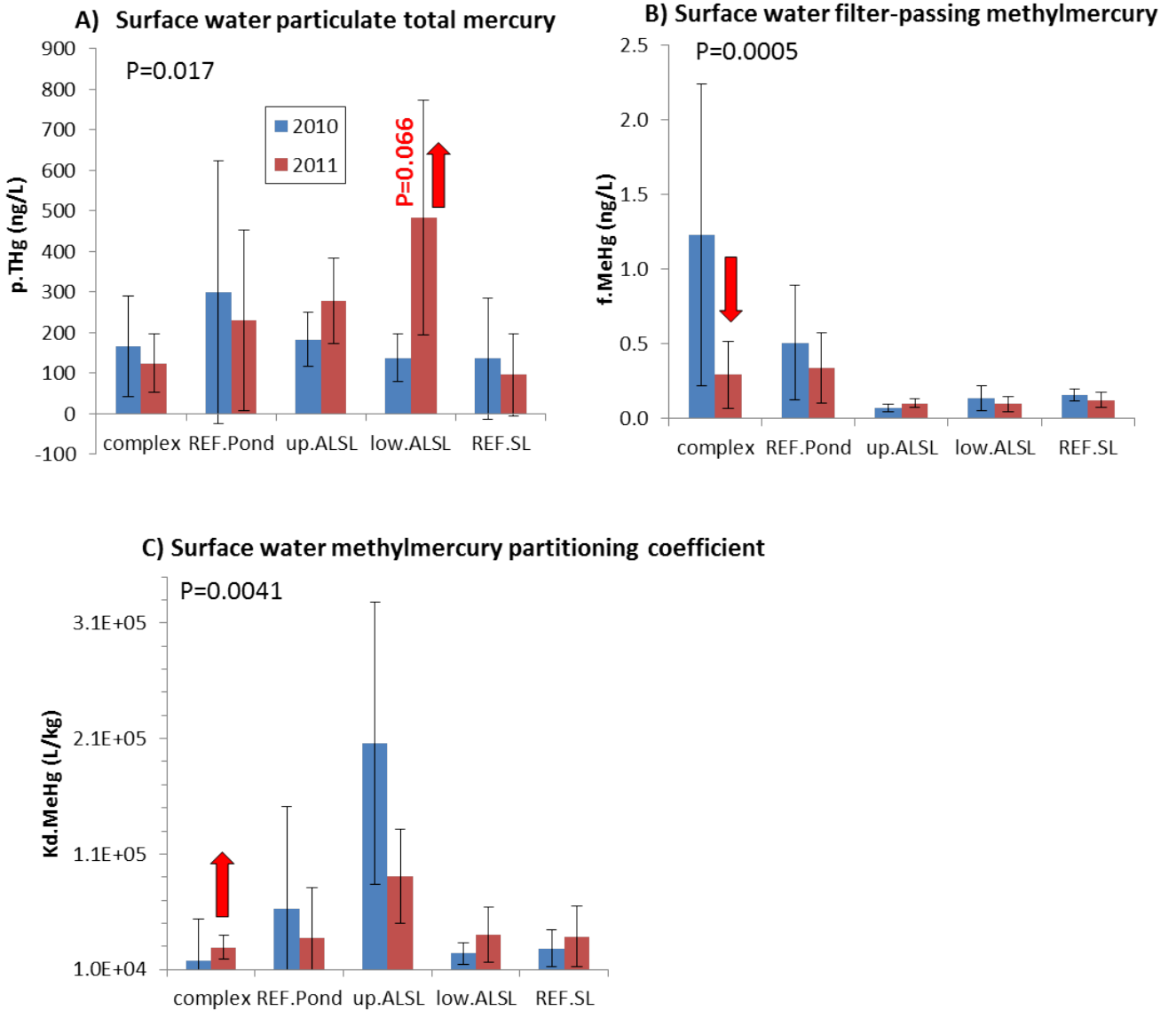
Figure 43. Bar graphs of mercury parameters in surface water by YEAR and LOCATION. Colored bars represent the mean and error bars represent the standard deviation. The statistical Probability (P) value associated with the global model YEAR*LOCATION interaction term is given for each parameter plot. Statistically significant differences ( P < 0.05 , unless otherwise noted) between YEARS for an individual LOCATION is indicated by the red arrow, as either an increase (up arrow) or decrease (down arrow) from 2010 to 2011. The specific sites associated with each LOCATION grouping are identified in Table 12.
