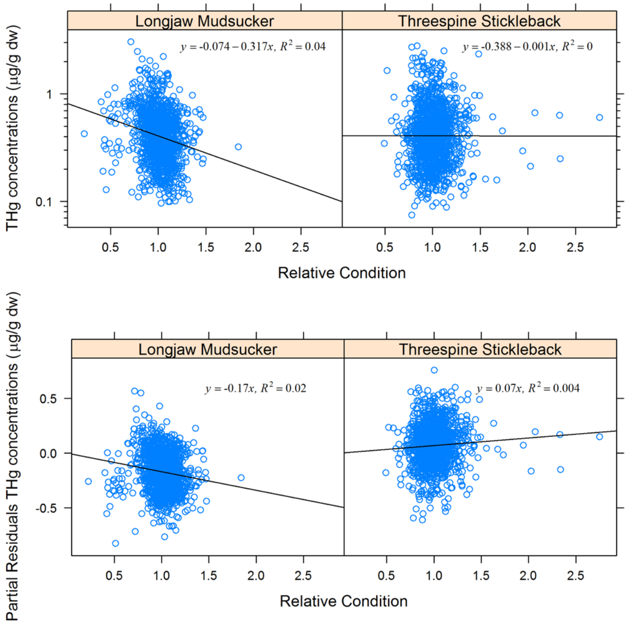
Figure 17. Longjaw Mudsucker and Threespine Stickleback total mercury (THg) concentrations ( \mu\text{g/g} dry weight) were poorly correlated with their relative body condition ( K_r ) within San Francisco Bay, CA. Top panel: Raw data. Lower panel: Partial residual plot after controlling for variation among pond sites, year, and date.
