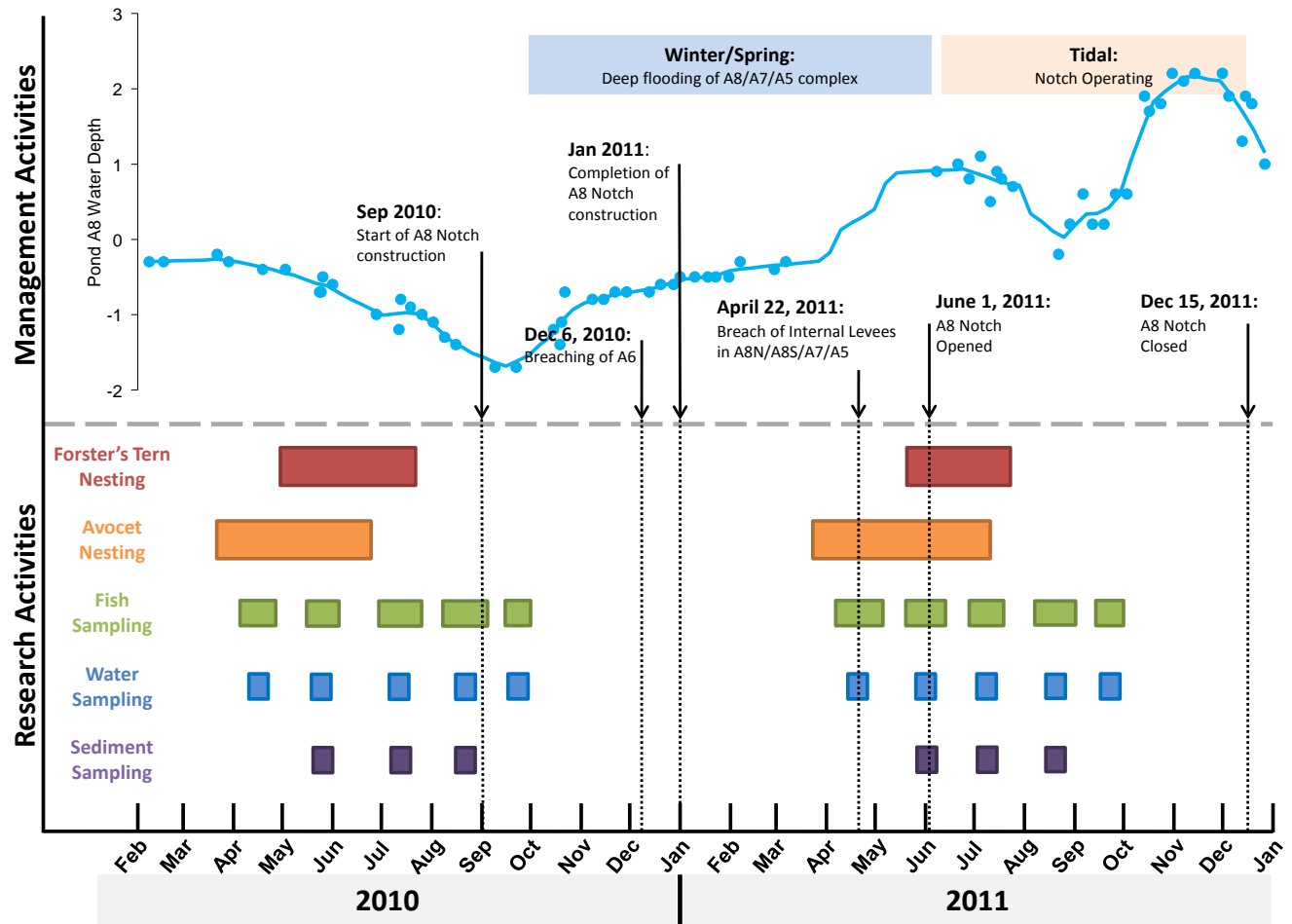
Figure 1. Timeline for management and science activities associated with the restoration of Pond A8 by the South Bay Salt Pond Restoration Project in South San Francisco Bay, CA.
