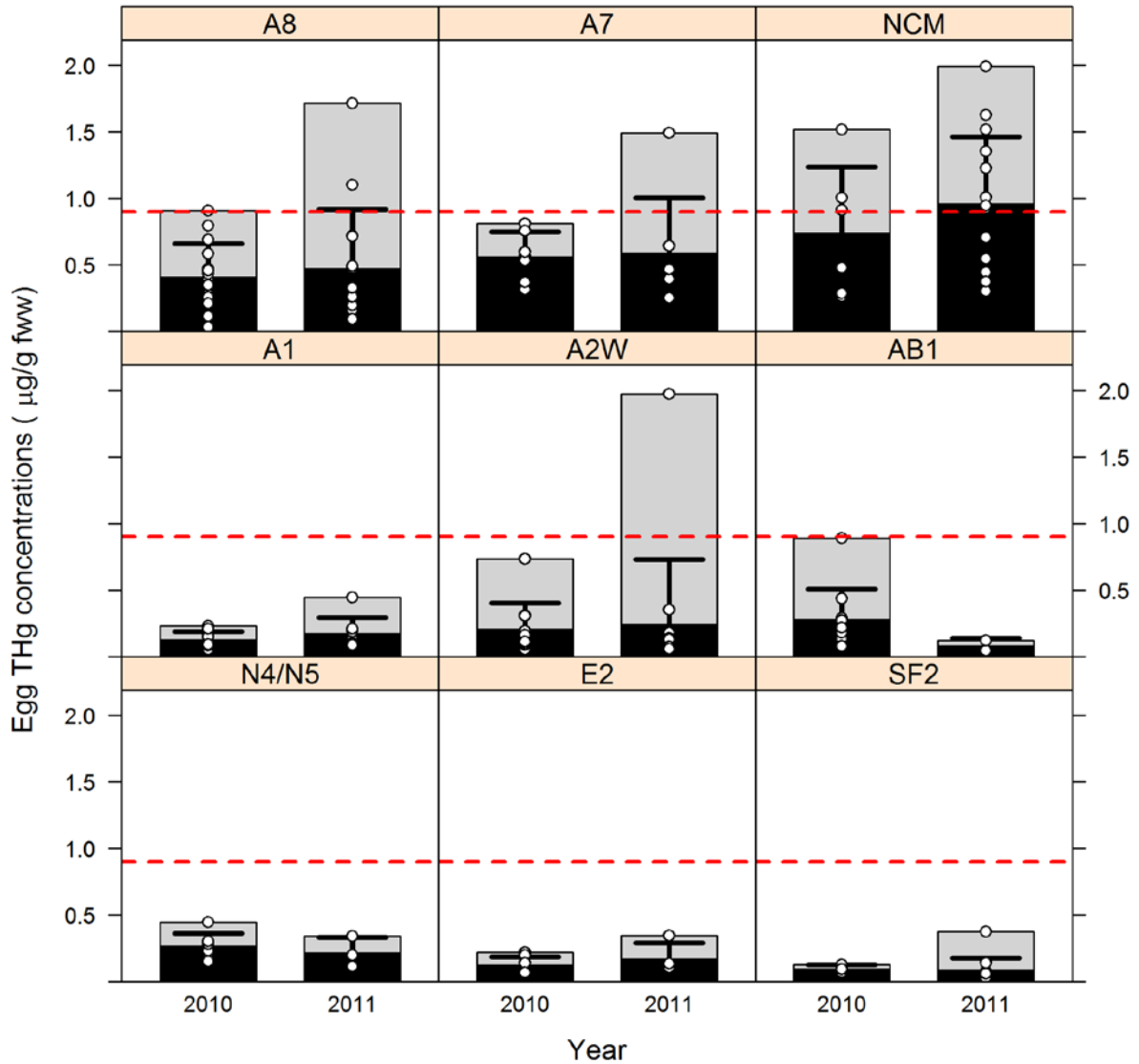
Figure 7. Pond site and year differences in egg mercury concentrations ( \mu\text{g/g fww} ) for American Avocets nesting in South San Francisco Bay Restoration Project area. Black bar represents arithmetic mean egg mercury concentrations. The error bar represents the standard deviation of the data. Gray box indicates the maximum egg mercury concentration observed. The white circles display the actual mercury concentration for each individual egg. The red dashed line displays the toxicity threshold of 0.90 \mu\text{g/g fww} where bird reproduction is impaired (Ackerman and Eagles-Smith 2008).
