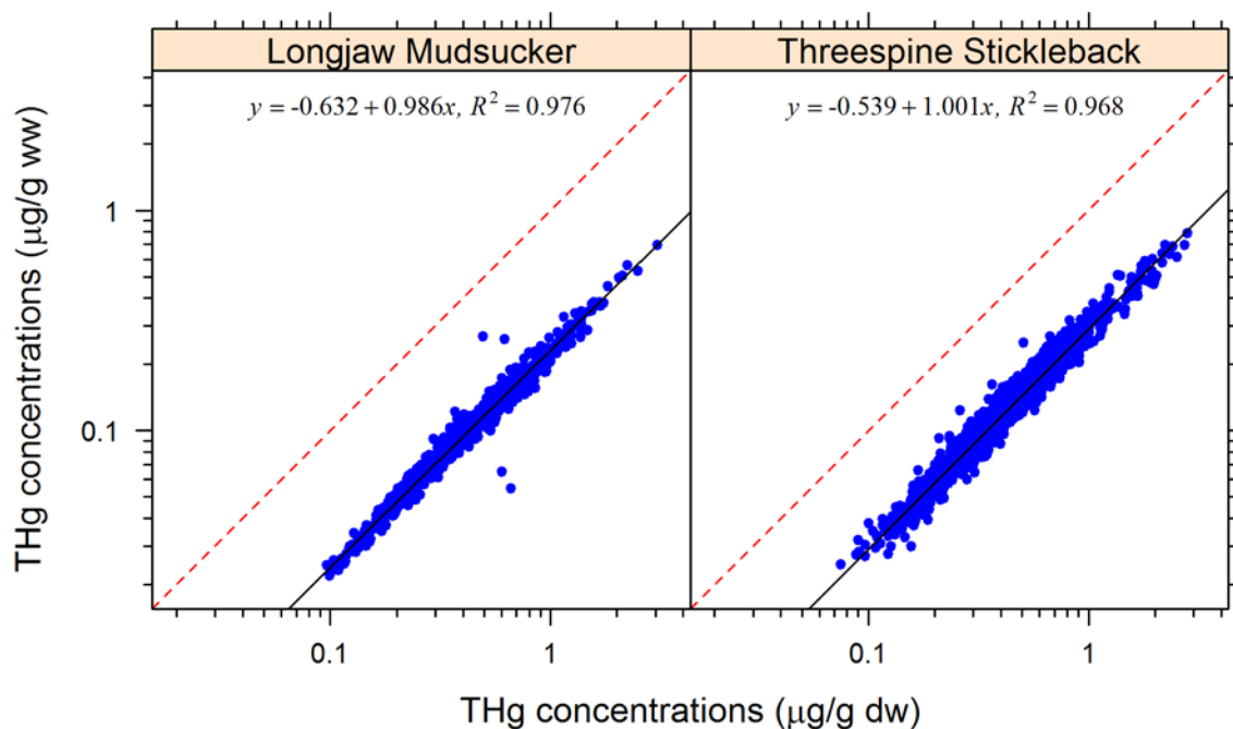
Figure 12. Total mercury (THg) concentrations on a wet weight basis ( \mu\text{g/g} wet weight) were highly correlated with THg concentrations on a dry weight basis ( \mu\text{g/g} dry weight) in both Longjaw Mudsucker (left panel) and Threespine Stickleback (right panel), although the slopes of the regressions differed between species.
