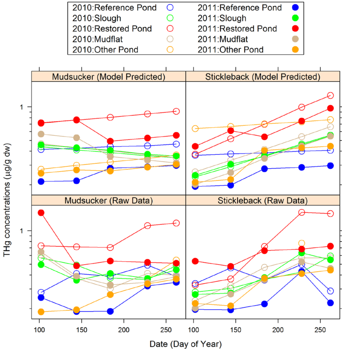
Figure 26. Changes in Mudsucker (left panels) and Stickleback (right panels) total mercury (THg) concentrations ( \mu\text{g/g} dry weight) are presented as model-averaged predictions (top panels) and summarized raw data (bottom panels). In 2010, Reference Ponds (open blue circles), showed an increase in THg concentrations over time (April – October) for both species. A similar relationship was seen in 2011 (solid blue circles), but at lower overall THg concentrations. In 2010, Restored Ponds (open red circles) had higher THg concentrations, but showed the same general trend over time. In 2011, Restored Ponds (solid red circles) began the season with higher THg concentrations, indicating that the restoration actions likely increased fish THg concentrations. In addition, Restored Ponds in 2011 exhibited a decrease in THg in early June, not observed in the Reference Pond data. This suggests that the opening of the Pond A8 Notch on June 1, 2011 (day of year = 152) caused a reduction in fish THg concentrations, with Bay water, and its lower Hg concentrations, diluting the overall concentrations of Hg in the Restored Ponds – at least in the short term.
