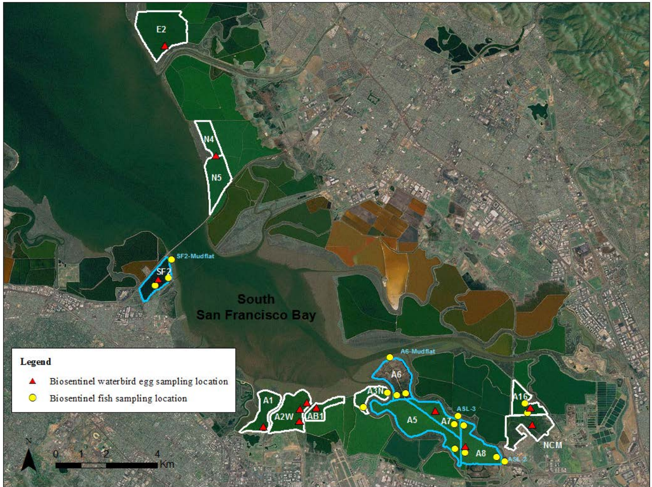
Figure 9. Sampling locations for mercury biosentinel bird eggs (red triangles) and fish (yellow circles) within Restored Ponds (A8, A7, and A5), Reference Ponds (A16, A3N, A1, A2W, AB1, N4/5, E2, and New Chicago Marsh), Restored Pond A6, Enhanced Pond SF2, A6 Mudflat, SF2 Mudflat, and two sites in Alviso Slough (below the Pond A8 Notch but above the Pond A6 breaches).
