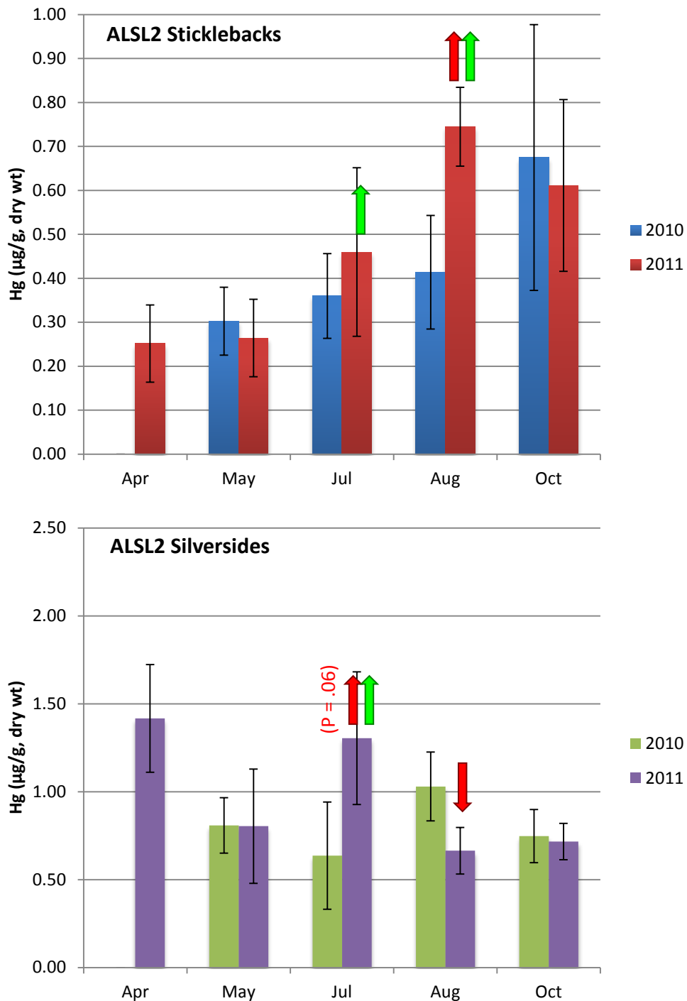
Figure 33. Site Alviso Slough 2 = ALSL2 (at Pond A8 notch location). Threespine Stickleback and Mississippi Silverside mean mercury concentrations \pm std. dev. THg ng/g dw, by month and year, before (2010) and after (2011) restoration activities. Note 2011 increases vs 2010 for Sticklebacks in July and August and for Silversides in July. Statistically significant differences ( P < 0.05 , except as indicated) between YEARS for the individual LOCATION is indicated by red arrow, as either an increase (up arrow) or decrease (down arrow) from 2010 to 2011. Green arrows indicate statistically sig. differences between years for the individual location in relation to corresponding trends at the control site (MALSL).
