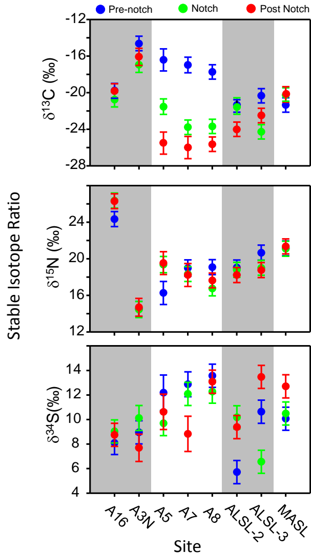
Figure 52. Stable carbon ( \delta^{13}\text{C} ), nitrogen ( \delta^{15}\text{N} ), and sulfur ( \delta^{34}\text{S} ) isotope ratios in Threespine Stickleback samples from sites in the South Bay Salt Pond Restoration Project. Dots represent mean values, error bars are standard error. Blue, green, and red symbols are from the "pre-notch", "notch", and "post-notch" time periods, respectively.
