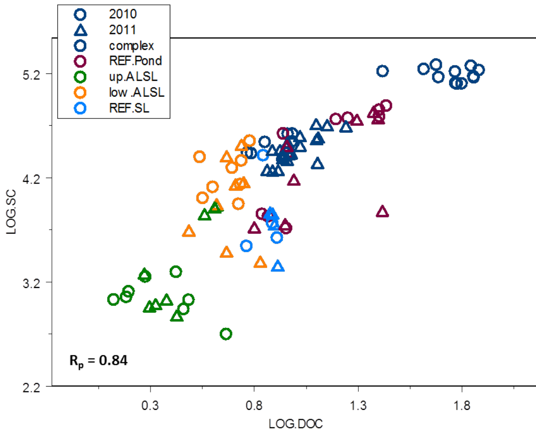
Figure 51. X-Y Scatter plot of surface water (LOG10 transformed) specific conductivity (S.C.) versus (LOG10 transformed) dissolved organic carbon (DOC). Symbols are coded by both YEAR and LOCATION. The Pearson's Correlation coefficient ( R_p ) is given.
