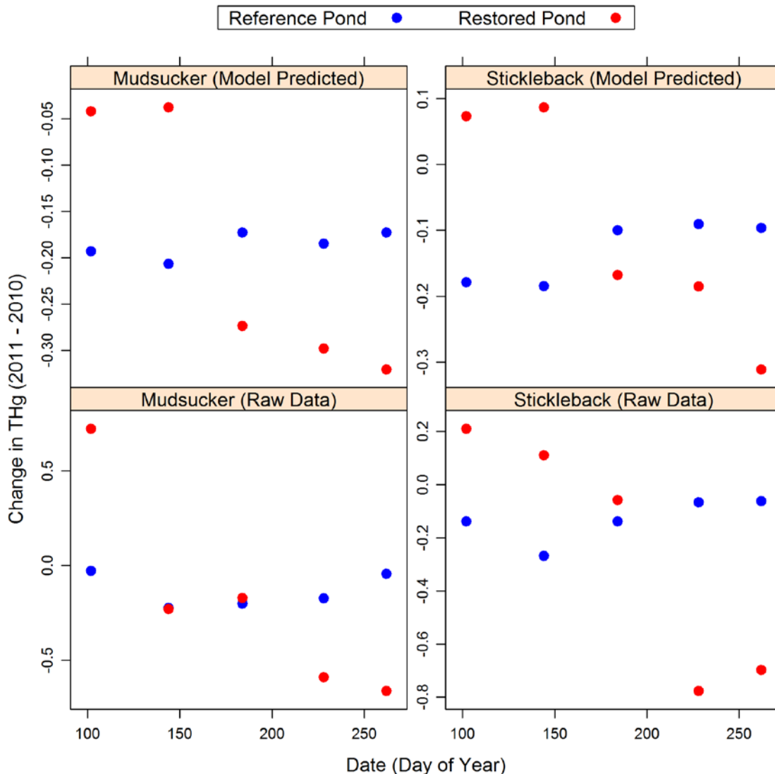
Figure 24. Difference between post-restoration (2011) and pre-restoration (2010) total mercury (THg) concentrations ( \mu\text{g/g} dry weight) versus sampling time period for Reference Ponds (blue: A16 and A3N) and Restored Ponds (red: A5, A7, and A8) in San Francisco Bay, CA. Longjaw Mudsucker data are presented on the left panels and Threespine Stickleback data are presented on the right panels. Raw data are presented on the bottom panels and model-predicted data, which account for other variables which influenced THg concentrations in fish, are presented on the top panels. Whereas most of the management activities associated with the restoration of the Pond A8/A7/A5 Complex occurred between years of sampling, the Pond A8 Notch was physically opened to tidal influence on June 1, 2011 (day of year = 152), between sampling time periods two and three in 2011. The data show that for both Mudsuckers and Stickleback, fish THg concentrations increased, relative to Reference Ponds, after the restoration activities between years for the first two sampling time periods before the Pond A8 Notch was opened in 2011. However after the Pond A8 Notch was opened, fish THg concentrations declined in Restored Ponds relative to Reference Ponds.
