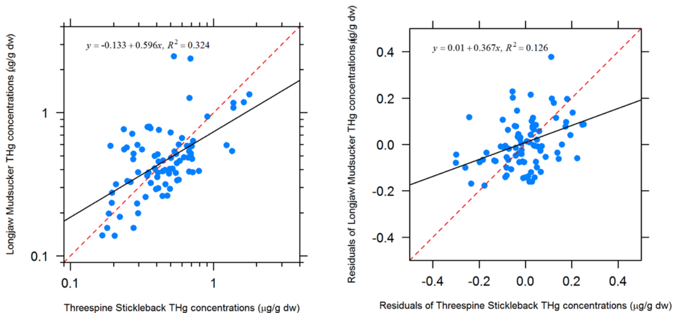
Figure 18. Total mercury (THg) concentrations ( \mu\text{g/g} dry weight) in Longjaw Mudsucker were somewhat correlated with THg concentrations ( \mu\text{g/g} dry weight) in Threespine Sticklebacks within San Francisco Bay, CA. Left panel: Correlation in raw data. Right panel: Correlation in residuals after controlling for variation of THg among pond sites, year, date, and fish length. Each data point represents mean fish mercury concentrations for each group of fish identified by species, pond, and sampling time period.
