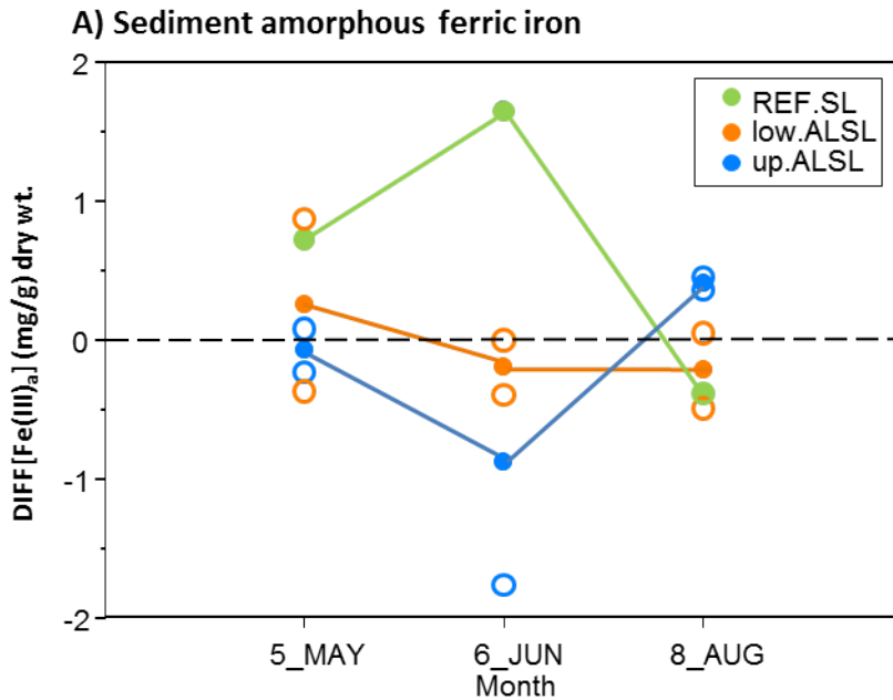
Figure 41. Line graph of the annual difference (DIFF[Y2011 – Y2010]) for non-mercury parameters in surface sediment of Sloughs, by MONTH and LOCATION. Open circles represent the original data, while closed circles with lines represent the DIFF-Y model predicted values, where DIFF-Y = MONTH + LOCATION + MONTH*LOCATION . Only cases where a Tukey's family-wise comparison of LOCATION resulted in significant differences ( P < 0.05 ) between the reference location (REF.Slough) and the treatment location (up.ALSL and/or low.ALSL) are depicted. The specific sites associated with each LOCATION grouping are identified in Table 10. The results indicate that for at least one of the sampling months the interannual variability in sediment amorphous ferric iron ( Fe(III)_a ) was significantly different between the REF.SL and the two Alviso Slough LOCATIONS, with a notable increase in Fe(III)_a between 2010 and 2011 during June.
