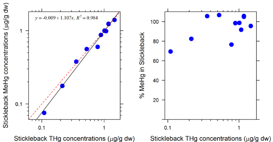
Figure 14. Left Panel: Threespine Stickleback methylmercury (MeHg) concentrations (µg/g dry weight) were highly correlated with total mercury (THg) concentrations (µg/g dry weight) within San Francisco Bay salt ponds. Right Panel: Percentage of total mercury (THg) in the methylmercury form (MeHg) was not related to THg concentrations (µg/g dry weight) in Threespine Stickleback within San Francisco Bay salt ponds.
