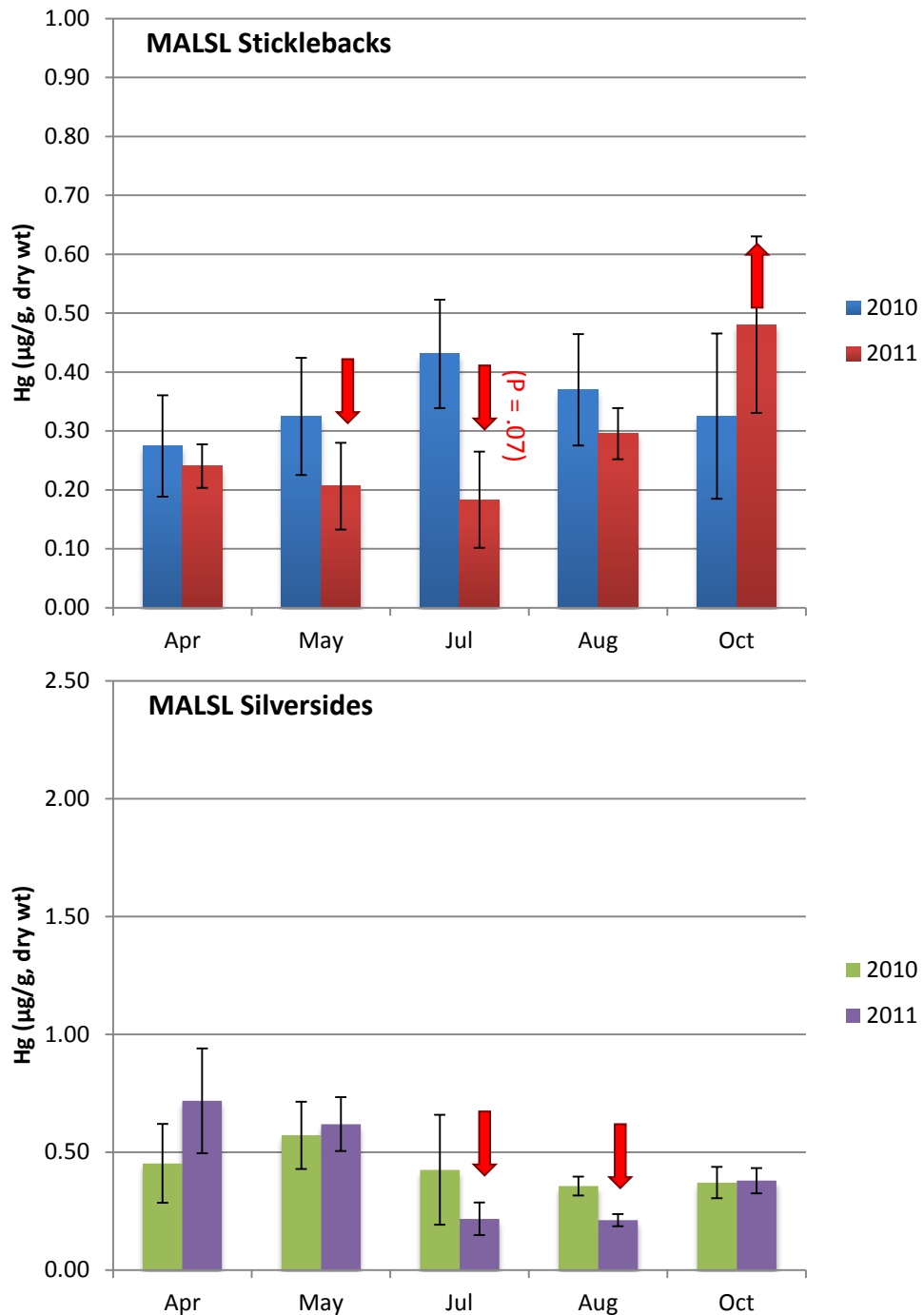
Figure 31. Site Mallard Slough = MALSL (control site away from Alviso Slough). Note generally lower concentrations than Alviso Slough sites (Figs. 32-35) and steady or declining interannual trends May through August of 2011 vs 2010. Threespine Stickleback and Mississippi Silverside mean mercury concentrations \pm std. dev. THg \mu\text{g/g} dry weight, by month and year. Statistically significant differences ( P < 0.05 , except as indicated) between YEARS for the individual LOCATION is indicated by the red arrow, as either an increase (up arrow) or decrease (down arrow) from 2010 to 2011.
