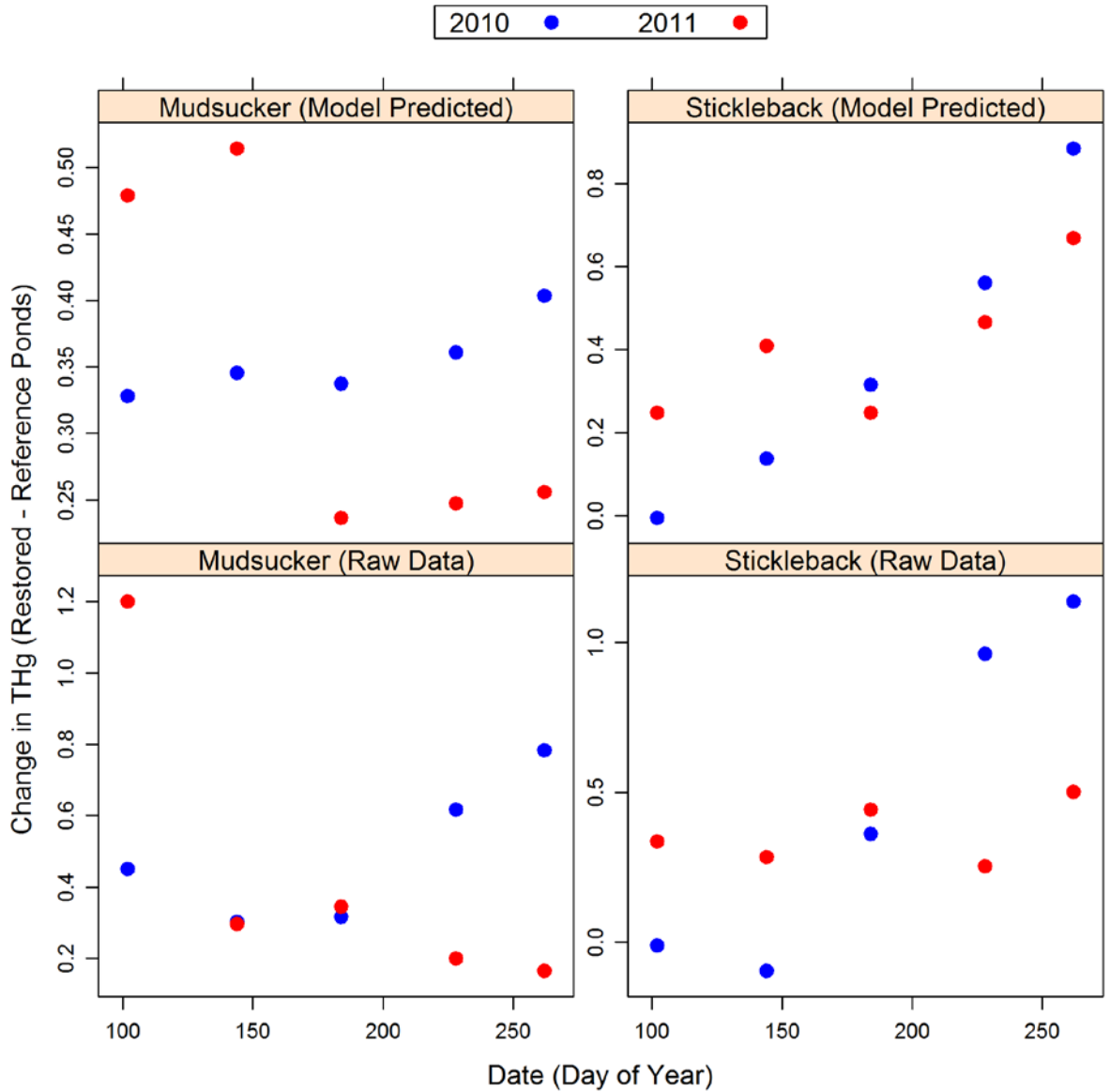
Figure 25. Difference between Restored Pond (A5, A7, and A8) and Reference Pond (A16 and A3N) total mercury (THg) concentrations ( \mu\text{g/g} dry weight) versus sampling time period for pre-restoration (blue: 2010) and post-restoration (red: 2011) in San Francisco Bay, CA. Longjaw Mudsucker data are presented on the left panels and Threespine Stickleback data are presented on the right panels. Raw data are presented on the bottom panels and model predicted data, which account for other variables which influenced total mercury concentrations in fish, are presented on the top panels. Whereas most of the management activities associated with the restoration of the Pond A8/A7/A5 Complex occurred between years of sampling, the Pond A8 Notch was physically opened to tidal influence on June 1, 2011 (day of year = 152), between sampling time periods two and three in 2011. The data show that for both Mudsuckers and Stickleback, fish THg concentrations increased, relative to Reference Ponds, after the restoration activities between years for the first two sampling time periods before the Pond A8 Notch was opened in 2011. However after the Pond A8 Notch was opened, fish THg concentrations declined in Restored Ponds relative to Reference Ponds.
