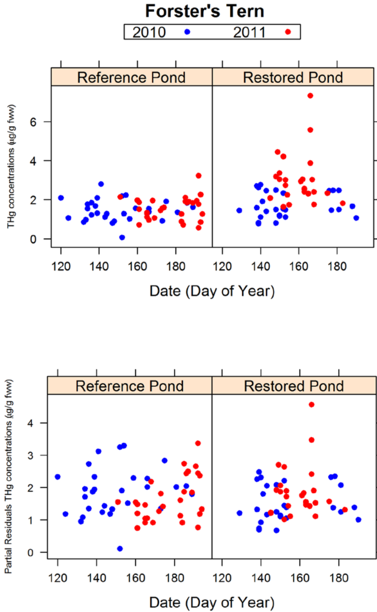
Figure 6. THg concentrations ( \mu\text{g/g fww} ) in Forster's Tern eggs by date within the South Bay Salt Pond Restoration Project area, before (2010: blue) and after (2011: red) the management activities associated with the restoration of the Pond A8/A7/A5 Complex in Fall 2010 through Spring 2011. The Pond A8 Notch was opened on June 1, 2011, corresponding to a potential exposure to eggs by June 8, 2011 (day of year = 159). The top panels display the raw data and the bottom panels display the partial residuals from the model.
