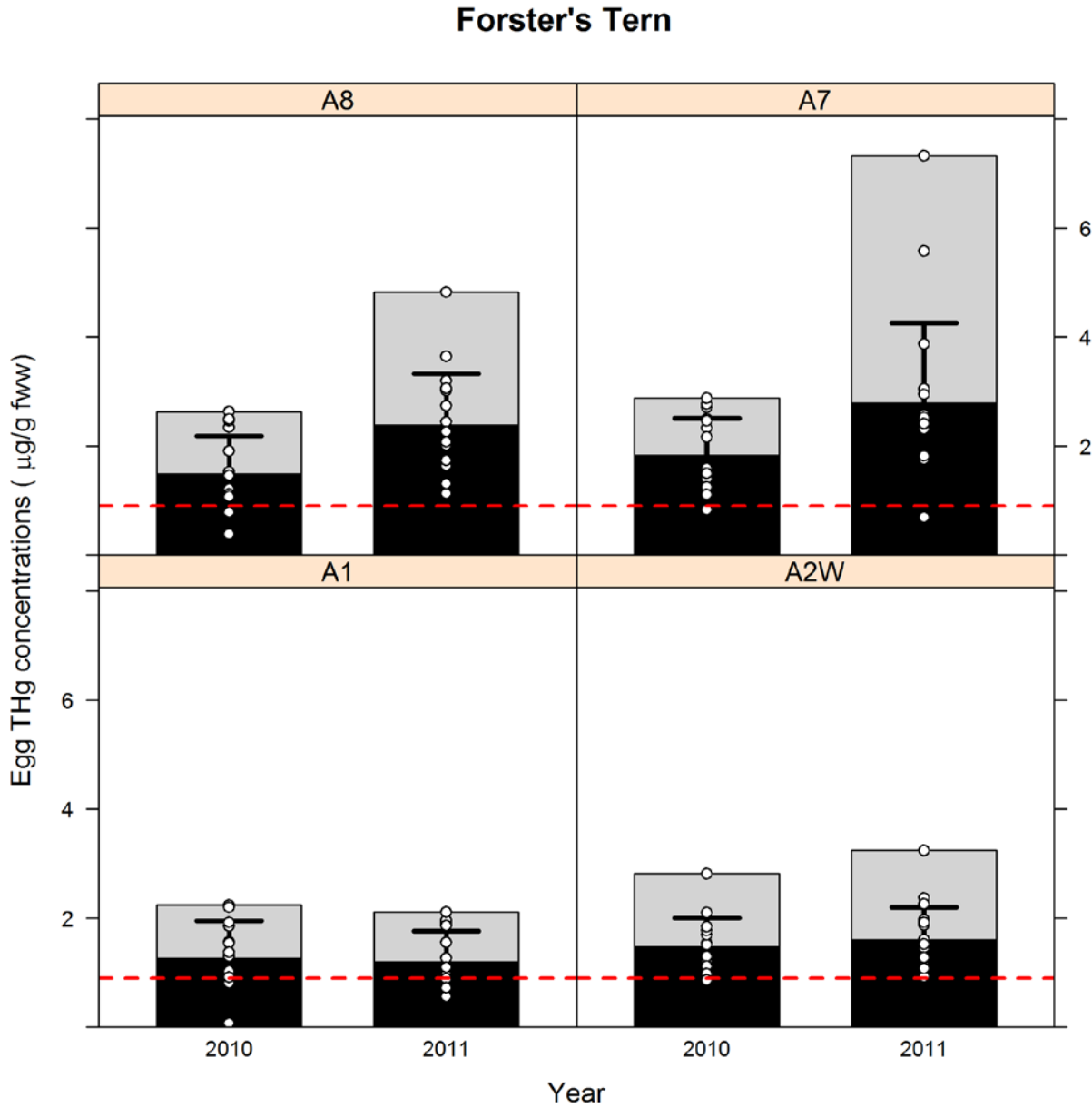
Figure 5. Pond site and year differences in egg mercury concentrations ( \mu\text{g/g fww} ) for Forster's Terns nesting in South San Francisco Bay Restoration Project area. Black bar represents arithmetic mean egg mercury concentrations. The error bar represents the standard deviation of the data. Gray box indicates the maximum egg mercury concentration observed. The white circles display the actual mercury concentration for each individual egg. The red dashed line displays the toxicity threshold of 0.90 \mu\text{g/g fww} where bird reproduction is impaired (Ackerman and Eagles-Smith 2008).
