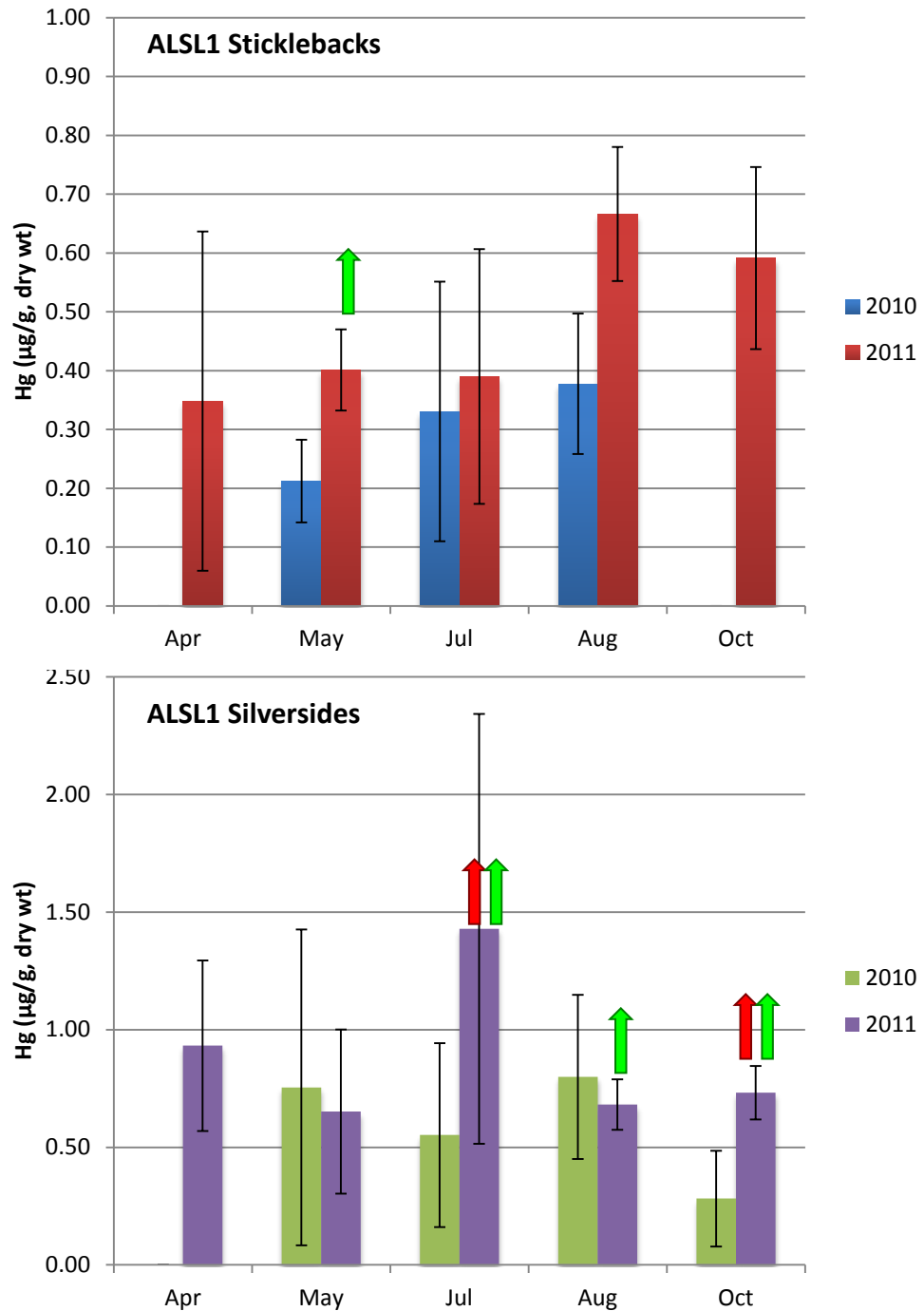
Figure 32. Site Alviso Slough 1 = ALSL1 (up-channel of Pond A8 notch location). Threespine Stickleback and Mississippi Silverside mean mercury concentrations \pm std. dev. Note 2011 increases vs 2010 for Sticklebacks in May and August and for Silversides in July. THg \mu\text{g/g} dry weight, by month and year, before (2010) and after (2011) restoration activities. Statistically significant differences ( P < 0.05 ) between YEARS for the individual LOCATION is indicated by the red arrow, as either an increase (up arrow) or decrease (down arrow) from 2010 to 2011. Green arrows indicate statistically significant differences between years for the individual location in relation to corresponding trends at the control site (MALSL).
