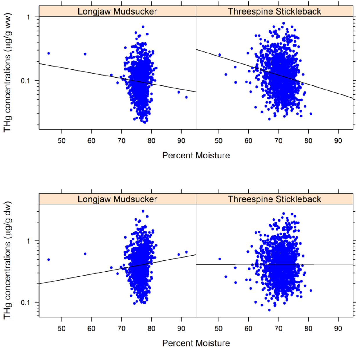
Figure 13. Top Panel: Fish total mercury (THg) concentrations in relation to percent moisture on a wet weight basis ( \mu\text{g/g} wet weight). Bottom Panel: Fish total mercury (THg) concentrations in relation to percent moisture on a dry weight basis ( \mu\text{g/g} dry weight).
