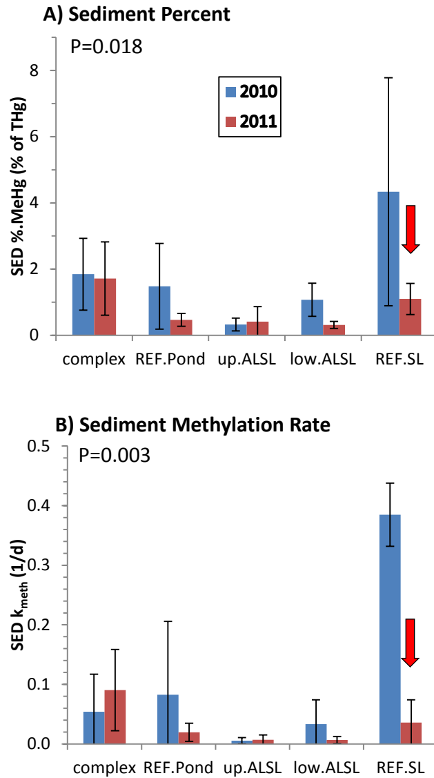
Figure 38. Bar graphs of mercury parameters in surface sediment by YEAR and LOCATION. Colored bars represent the mean and error bars represent the standard deviation. The statistical Probability (P) value associated with the global model YEAR*LOCATION interaction term is given for each parameter plot. Statistically significant differences ( P < 0.05 ) between YEARS for an individual LOCATION is indicated by the red arrow, as either an increase (up arrow) or decrease (down arrow) from 2010 to 2011. The specific sites associated with each LOCATION grouping are identified in Table 10.
