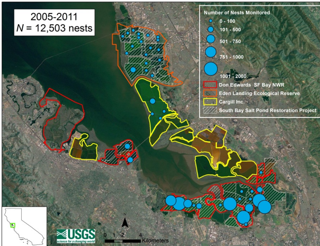
Figure 3. Locations of nesting Forster’s Terns and American Avocets within the South Bay Salt Pond Restoration Project area (from Ackerman and Herzog 2012).
