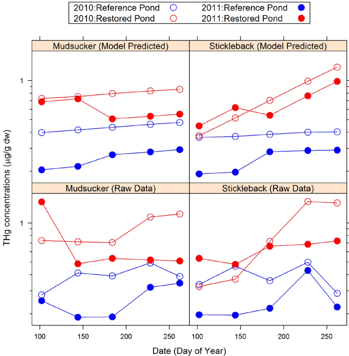
Figure 23. Changes in Mudsucker (left panels) and Stickleback (right panels) total mercury (THg) concentrations ( \mu\text{g/g} dry weight) are presented as model-averaged predictions (top panels) and summarized raw data (bottom panels). In 2010, Reference Ponds (open blue circles), showed an increase in THg concentrations over time (April – October) for both species. A similar relationship was seen in 2011 (solid blue circles), but at lower overall THg concentrations. In 2010, Restored Ponds (open red circles) had higher THg concentrations, but showed the same general trend over time. In 2011, Restored Ponds (solid red circles) began the season with higher THg concentrations, indicating that the restoration actions likely increased fish THg concentrations. In addition, Restored Ponds in 2011 exhibited a decrease in THg in early June, not observed in the Reference Pond data. This suggests that the opening of the Pond A8 Notch on June 1, 2011 (day of year = 152) caused a reduction in fish THg concentrations, with Bay water, and its lower Hg concentrations, diluting the overall concentrations of Hg in the Restored Ponds – at least in the short term.
