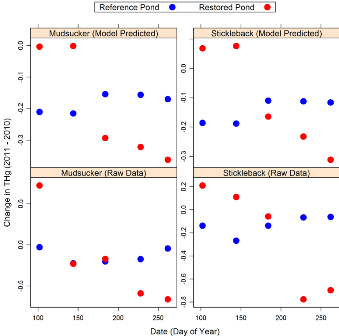
Figure 27. Difference between post-restoration (2011) and pre-restoration (2010) total mercury (THg) concentrations ( \mu\text{g/g} dry weight) versus sampling time period for Reference Ponds (blue: A16 and A3N) and Restored Ponds (red: A5, A7, and A8) in San Francisco Bay, CA. Longjaw Mudsucker data are presented on the left panels and Threespine Stickleback data are presented on the right panels. Raw data are presented on the bottom panels and model-predicted data, which account for other variables which influenced THg concentrations in fish, are presented on the top panels. Whereas most of the management activities associated with the restoration of the Pond A8/A7/A5 Complex occurred between years of sampling, the Pond A8 Notch was physically opened to tidal influence on June 1, 2011 (day of year = 152), between sampling time periods two and three in 2011. The data show that for both Mudsuckers and Stickleback, fish THg concentrations increased, relative to Reference Ponds, after the restoration activities between years for the first two sampling time periods before the Pond A8 Notch was opened in 2011. However after the Pond A8 Notch was opened, fish THg concentrations declined in Restored Ponds relative to Reference Ponds.
