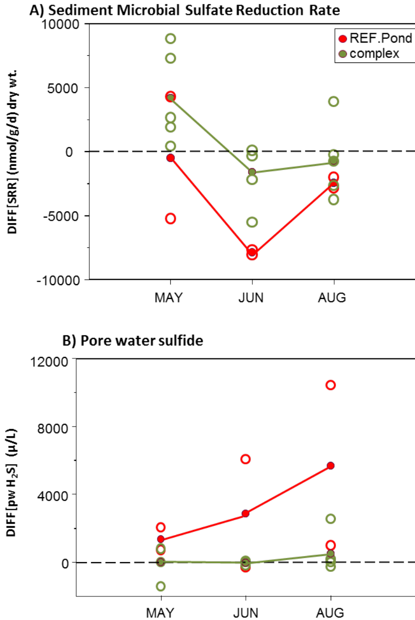
Figure 42. Line graphs of the annual difference (DIFF[Y2011 – Y2010]) for non-mercury parameters in surface sediment of Ponds, by MONTH and LOCATION. Open circles represent the original data, while closed circles with lines represent the DIFF-Y model predicted values, where DIFF-Y = MONTH + LOCATION + MONTH \times LOCATION . Only cases where a Tukey's family-wise comparison of LOCATION resulted in significant differences ( P < 0.05 ) between the reference location (REF.Pond) and the treatment location (A8/A7/A5 Ccomplex) are depicted. The specific sites associated with each LOCATION grouping are identified in Table 10. The results indicate that for at least one of the sampling months the interannual variability in both sediment SRR and pore water H_2S was significantly different between the REF.Pond and the Complex. There was a notable increase in sediment SRR for the Complex during May, and a decrease in SRR for the REF.Pond during June, between 2010 and 2011. There was also a notable increase in pore water H_2S for the REF.Pond during June and August, between 2010 and 2011.
