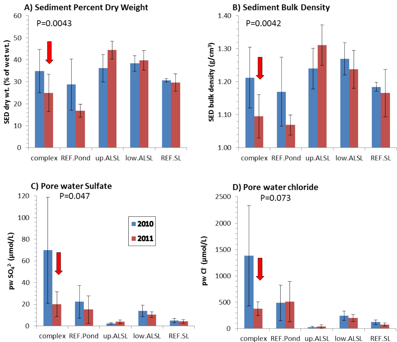
Figure 39. Bar graphs of non-mercury parameters in surface sediment and sediment pore water by YEAR and LOCATION. Colored bars represent the mean and error bars represent the standard deviation. The statistical Probability (P) value associated with the global model YEAR*LOCATION interaction term is given for each parameter plot. Statistically significant differences ( P < 0.05 ) between YEARS for an individual LOCATION is indicated by the red arrow, as either an increase (up arrow) or decrease (down arrow) from 2010 to 2011. The specific sites associated with each LOCATION grouping are identified in Table 10.
